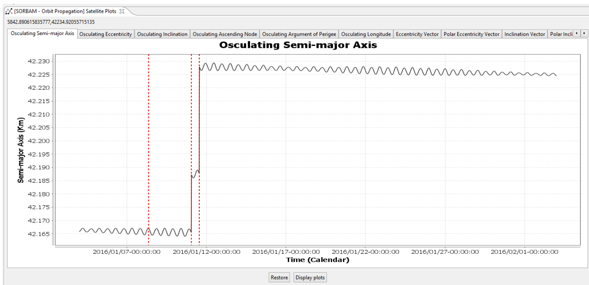
Figure 28 SORBAM Orbital evolution Plots (Osculating semi-major axis example)
