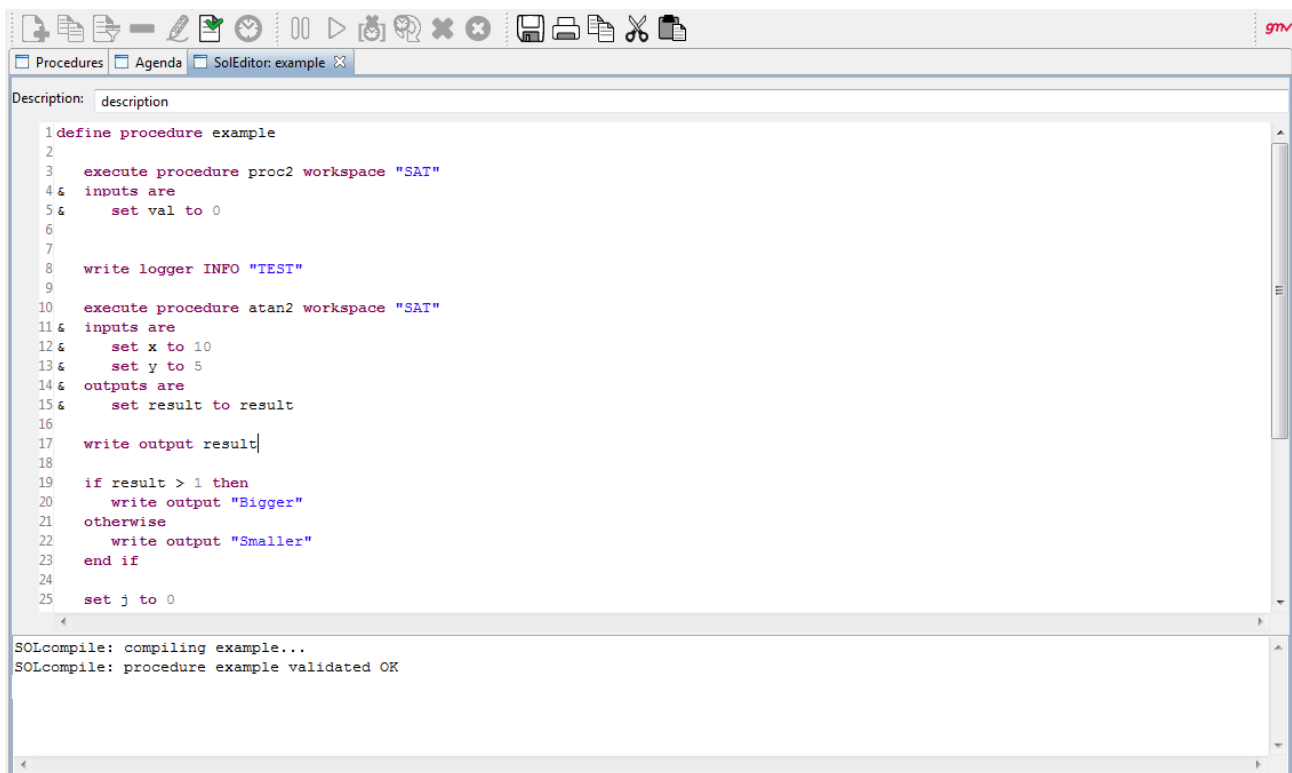
Figure 23: autofocus SOL Editor
