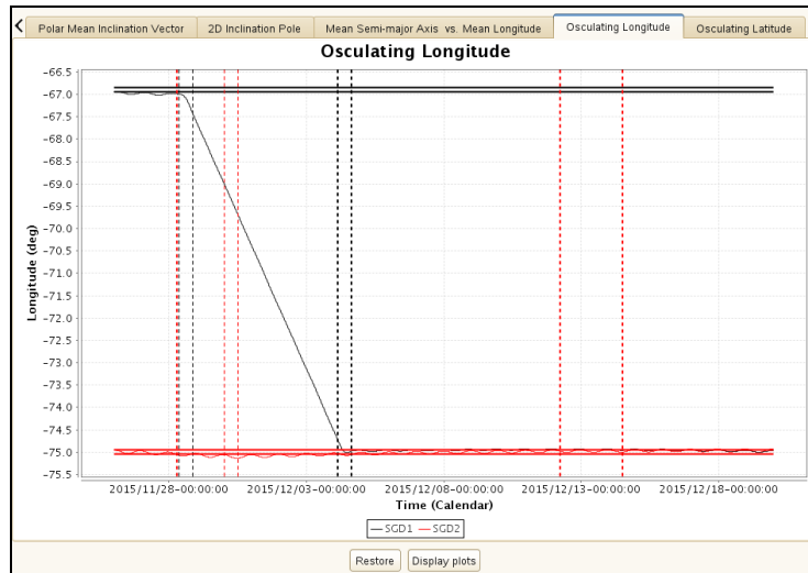
Figure 38: focusgeo INICOL Collocation Insertion Plot (Osculating longitude)
