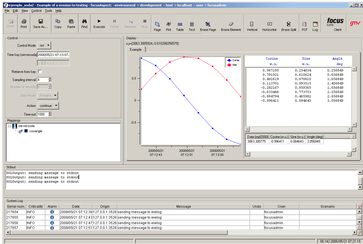
Figure 14: focusaspect Client main window
