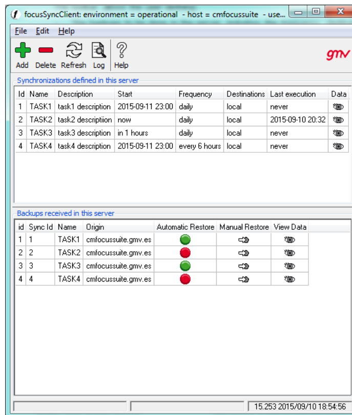
Figure 20: focussuitesync Client Main Window
