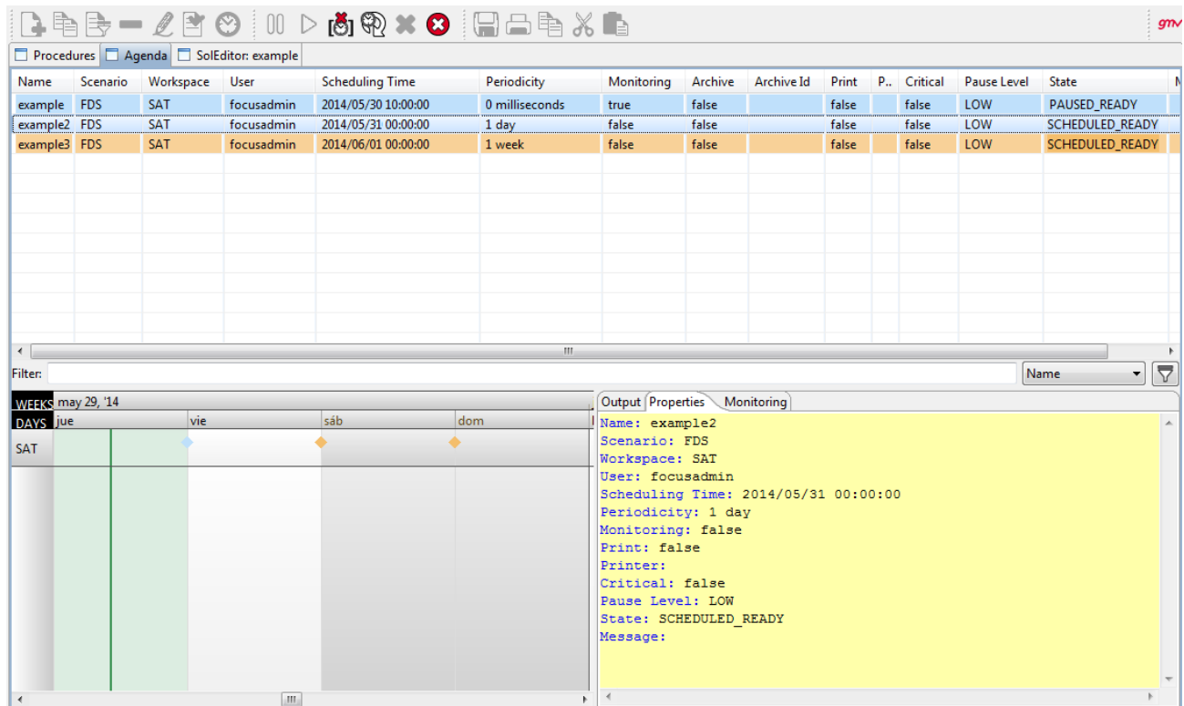
Figure 25: autofocus procedures agenda window
