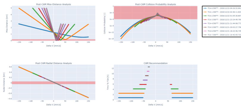
Figure 3. Collision Avoidance Manoeuvre Recommendation with Closeap
