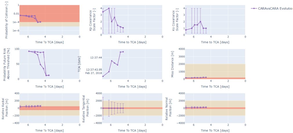
Figure 2. Conjunction Event Evolution with Closeap
