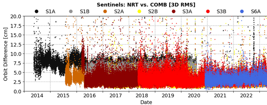
Fig. 18. Differences between CPOD NRT products and COMB solution in 3D RMS for Sentinel-1, –2, –3, and –6 missions.
