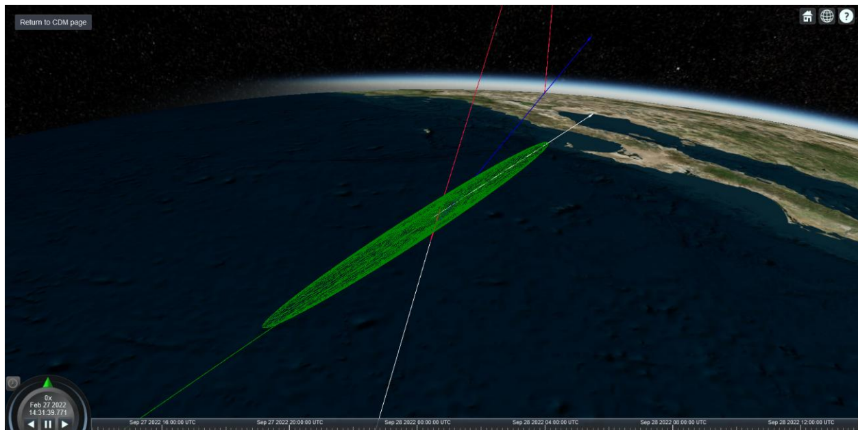
Figure 3: CDM covariance ellipsoid
