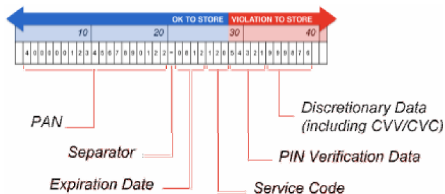
Figure 6: Track 2 Layout
